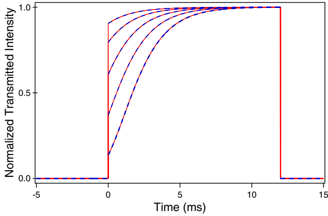
FIG. 5. Theoretical transmitted intensity as a function of time for an incident square pulse. Parameters are as follows: T_1 = 1.6 \mu\text{s} , \alpha L = 9 , \tau_{\text{in}} = 12 \text{ ms} , and, from top to bottom, I_0 = 0.1, 0.23, 0.5, 1 , and 2 . The solid and dashed lines are, respectively, the exact numerical solution and the approximate analytic solution given by Eq. (24).
