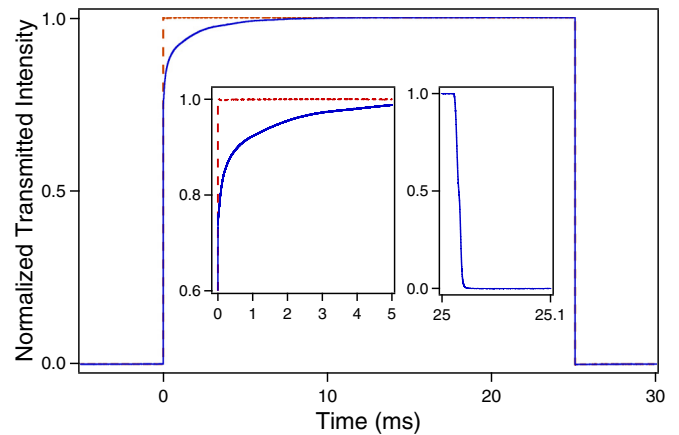
FIG. 4. Example of transmitted signal observed in our experiments for a power sent on the ruby crystal of about 1.6 W and a pulse duration \tau_{\text{in}} = 25 ms (solid line). The dashed line is the profile of the incident pulse obtained by replacing the ruby crystal by a suitable neutral density filter. The insets are enlargements of the pulse rise and fall.
