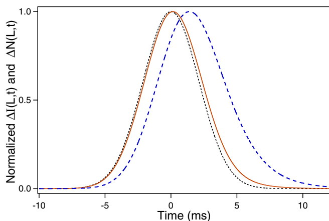
FIG. 1. Normalized transmitted pulse \Delta I(L,t) (solid line) and population variation \Delta N(L,t) (dashed line). Parameters are as follows: \bar{I}(0) = 0.23 , T_1 = 1.6 ms, \alpha = 1.17 cm ^{-1} , and L = 4.25 cm, leading to \alpha L \approx 5 , \bar{I}(L) \approx 2 \times 10^{-3} , T_L \approx T_1 , \Delta\tau_g(L) \approx T_1 , and \tau_{\text{gmod}}(L) \approx 0.3 ms. The normalized incident pulse \Delta I(0,t) (dotted line) of FWHM duration \tau_{\text{in}} = 5 ms is given for reference. Note the large delay of \Delta N(L,t) compared to that of \Delta I(L,t) .
