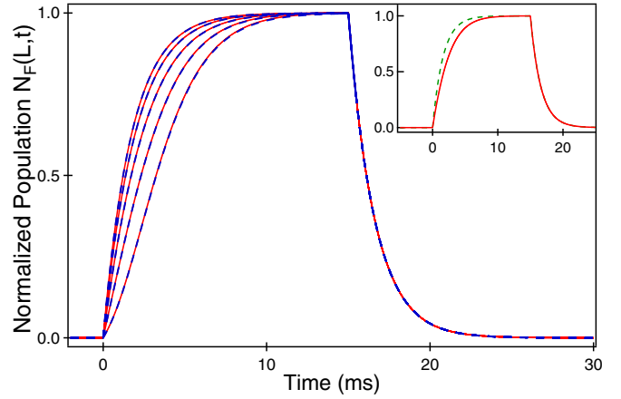
FIG. 6. Theoretical evolution of the fluorescent metastable level population. Pulse duration \tau_{\text{in}} = 15 \text{ ms} . Other parameters as in Fig. 5. The solid and dashed lines are, respectively, the exact numerical solution and the analytic solution given by Eqs. (26)–(28). (Inset) Comparison for I_0 = 0.5 of the exact numerical solution (solid line) to that given by Eqs. (28) and (29) analogous to those of an RC circuit (dashed line).
