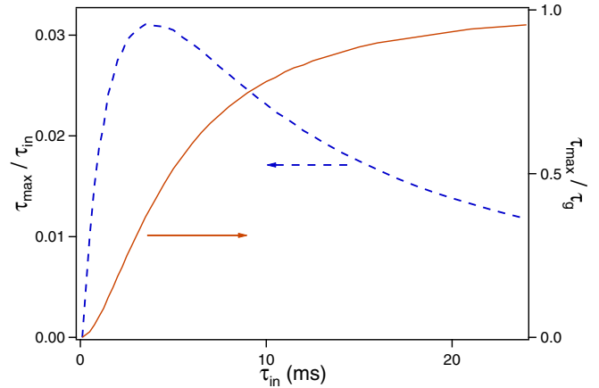
FIG. 2. Fractional delay \tau_{\max}/\tau_{\text{in}} of the transmitted pulse (dashed line, left scale) and ratio \tau_{\max}/\tau_{\text{gmod}} (solid line, right scale) as functions of the duration \tau_{\text{in}} of the incident pulse. Other parameters as in Fig. 1.
