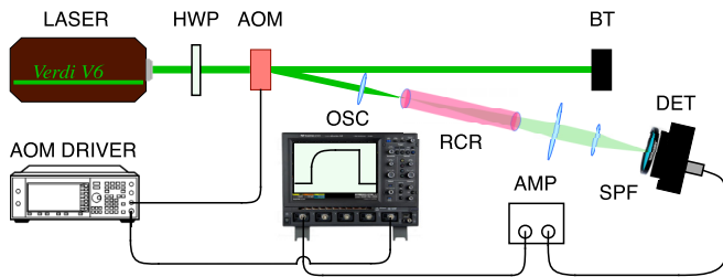
FIG. 3. Experimental setup. LASER, single longitudinal mode Nd:YVO 4 laser (Verdi V6, Coherent) delivering a cw at 532 nm; HWP, half-wave plate; AOM, acousto-optic modulator (AA Opto-Electronic, MTS110-A-VIS); BT, beam trap absorbing the non-diffracted light; RCR, ruby crystal rod; SPF, dichroic shortpass filter (Semrock, BSP-633R-25) eliminating the ruby fluorescence light at 694 nm; DET, high-speed silicon photodetector (Thorlabs DET 210, DC-350 MHz); AMP, low-band (DC-200 kHz) amplifier (Hamamatsu C7319); OSC, digital oscilloscope (Lecroy Waverunner 104 MXi); AOM DRIVER, function generator driving the acousto-optic modulator and triggering the oscilloscope.
